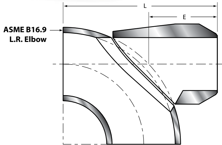
Low Weld Volume Butt-Weld Elbow Branchette® (LWV BEB)
