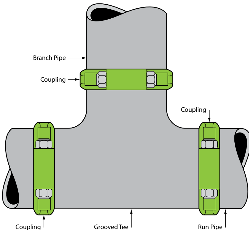
Conventional Grooved Tee
