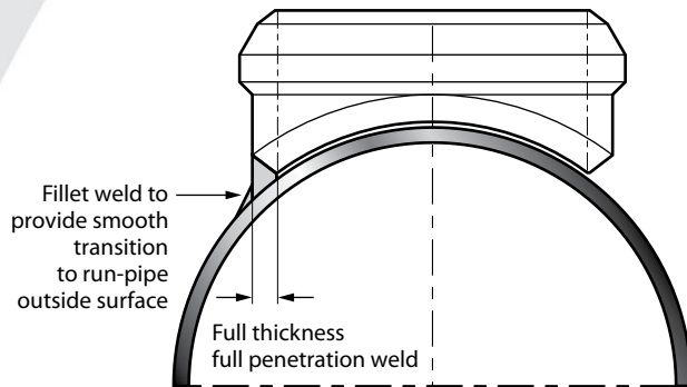
Transverse Section
