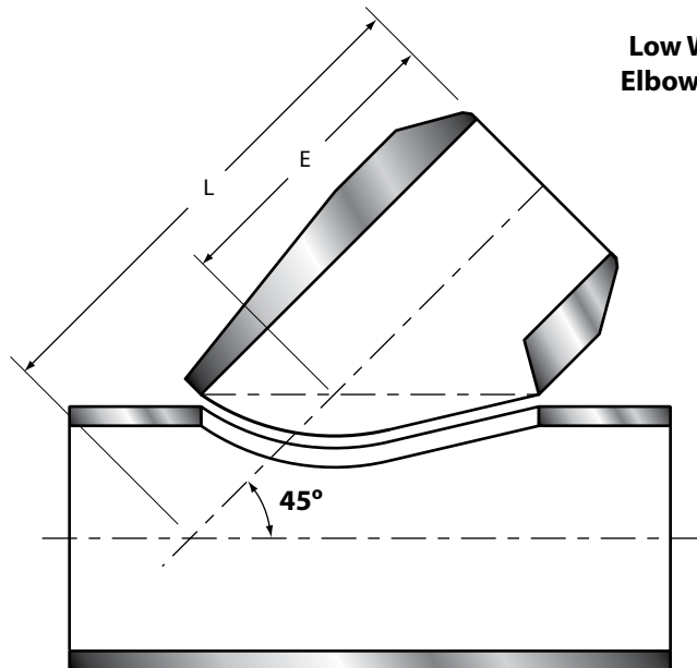
Low Weld Volume Butt-Weld 45° Lateral Branchette® (LWV BLB)
