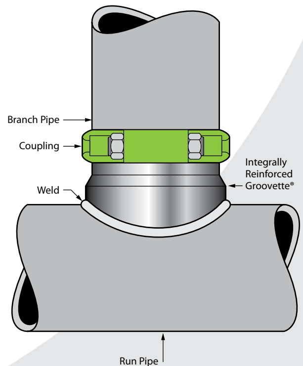
Integrally Reinforced Groovette®
