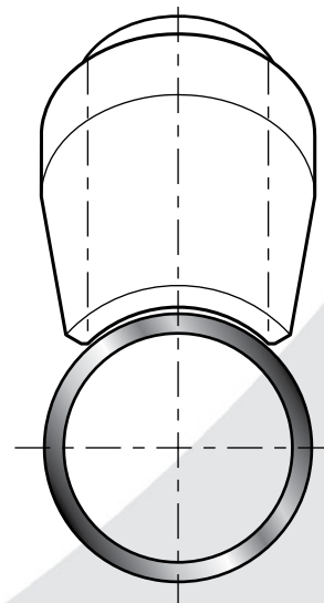
Low Weld Volume Butt-Weld 45° Lateral Branchette® (LWV BLB)
