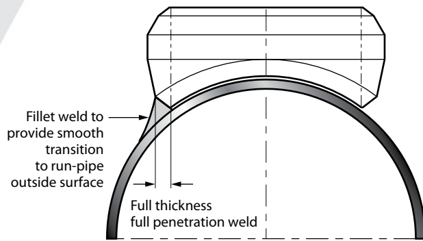
Transverse Section
