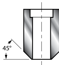
Socket-Weld Boss
