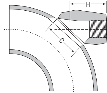
THREADED
