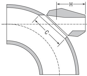
BUTTWELD
