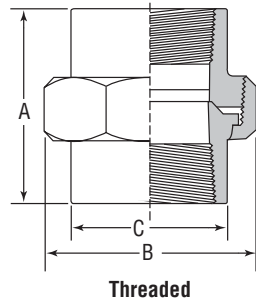
FIGURE 2125: Threaded Union
